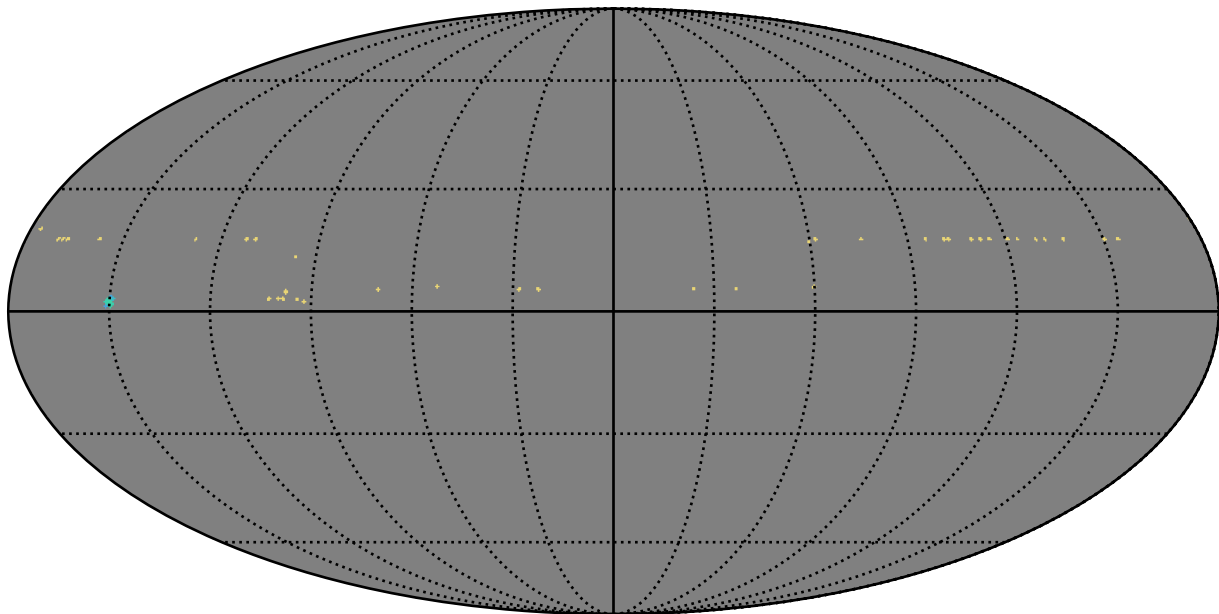
all_long_v3.4_10yrs y band: AGN_TimeLag_5_days
