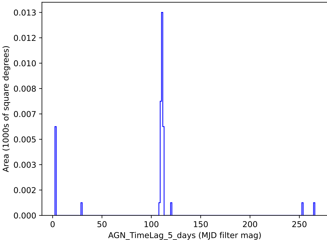
all_long_v3.4_10yrs y band: AGN_TimeLag_5_days
