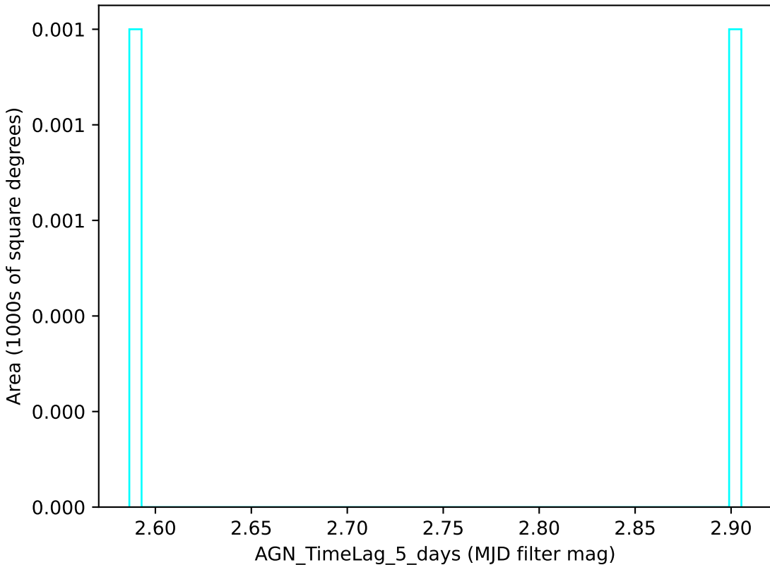
all_long_v3.4_10yrs u band: AGN_TimeLag_5_days
