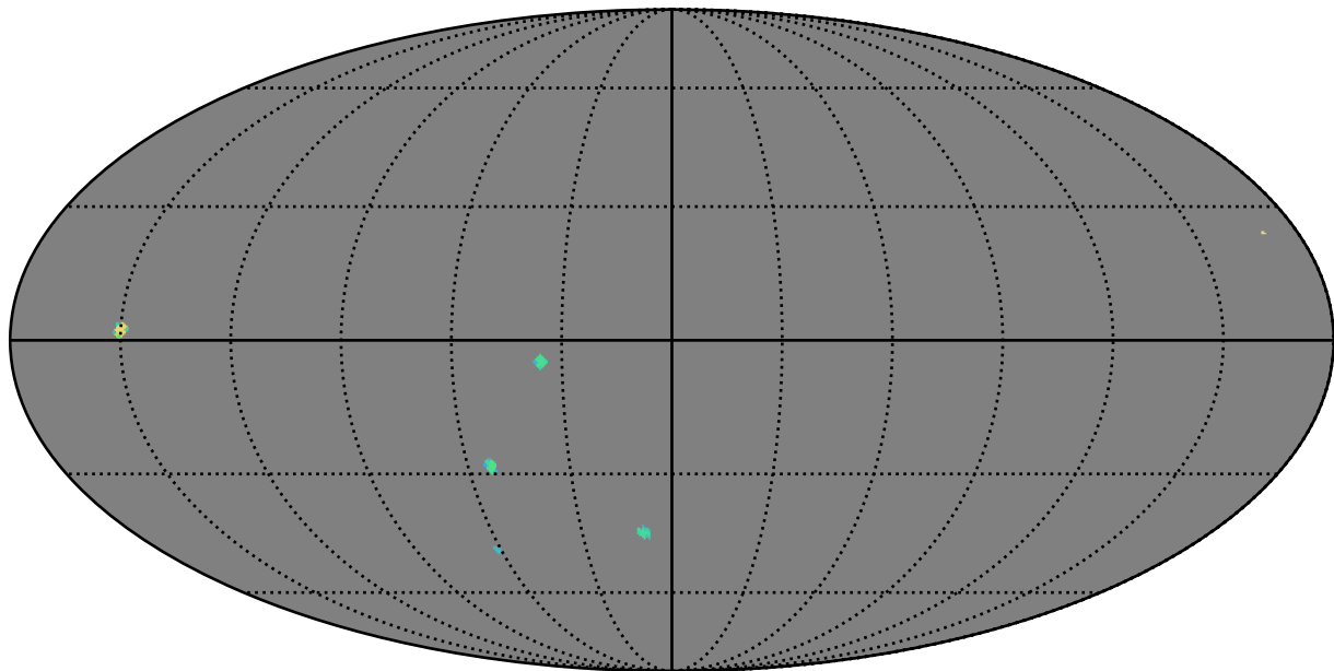
all_long_v3.4_10yrs r band: AGN_TimeLag_5_days
