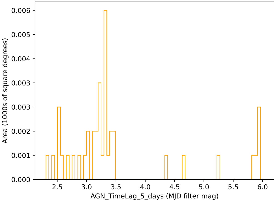
all_long_v3.4_10yrs r band: AGN_TimeLag_5_days
