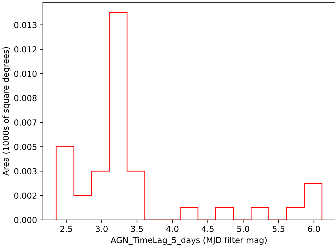
all_long_v3.4_10yrs i band: AGN_TimeLag_5_days
