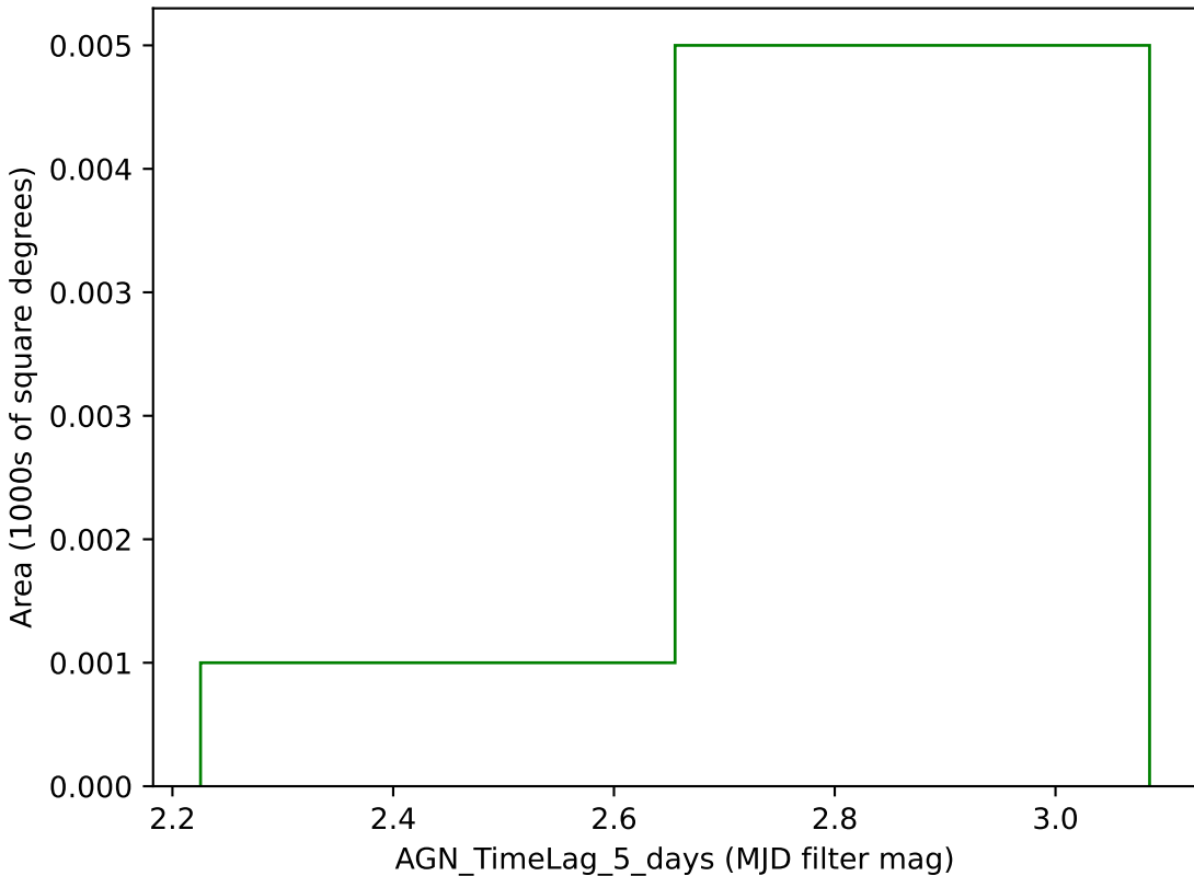
all_long_v3.4_10yrs g band: AGN_TimeLag_5_days
