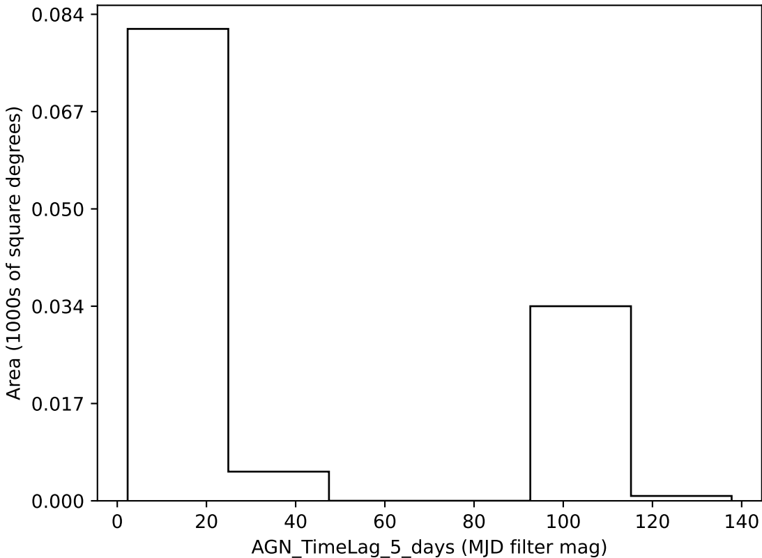
all_long_v3.4_10yrs all bands: AGN_TimeLag_5_days
