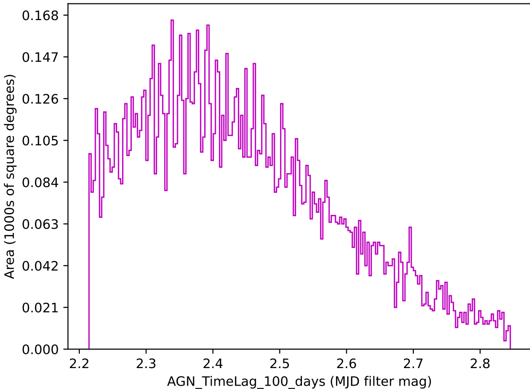
all_long_v3.4_10yrs z band: AGN_TimeLag_100_days
