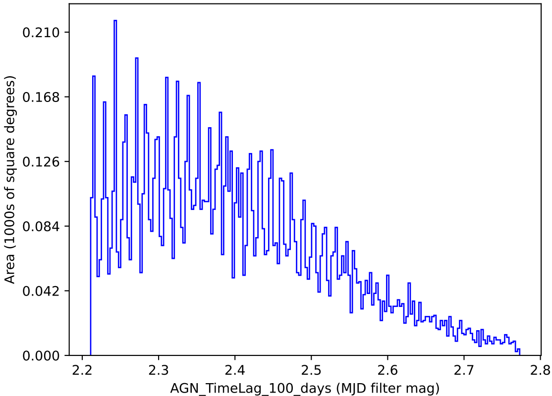
all_long_v3.4_10yrs y band: AGN_TimeLag_100_days
