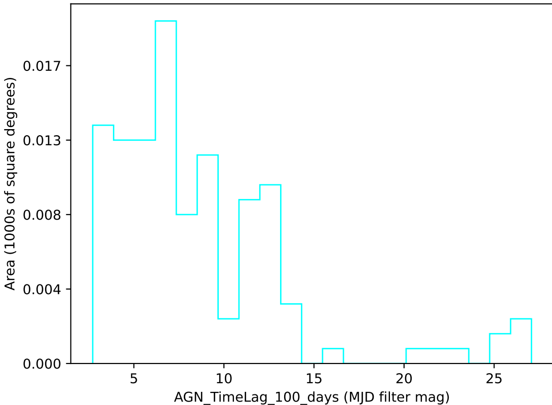
all_long_v3.4_10yrs u band: AGN_TimeLag_100_days
