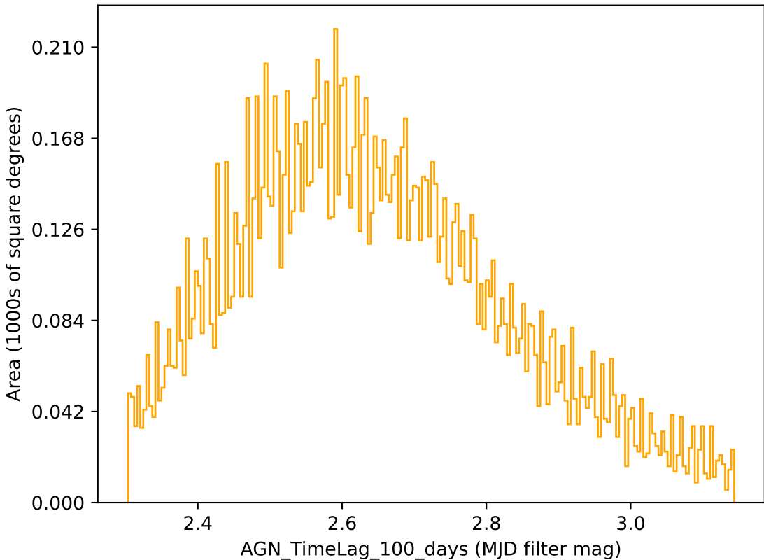
all_long_v3.4_10yrs r band: AGN_TimeLag_100_days
