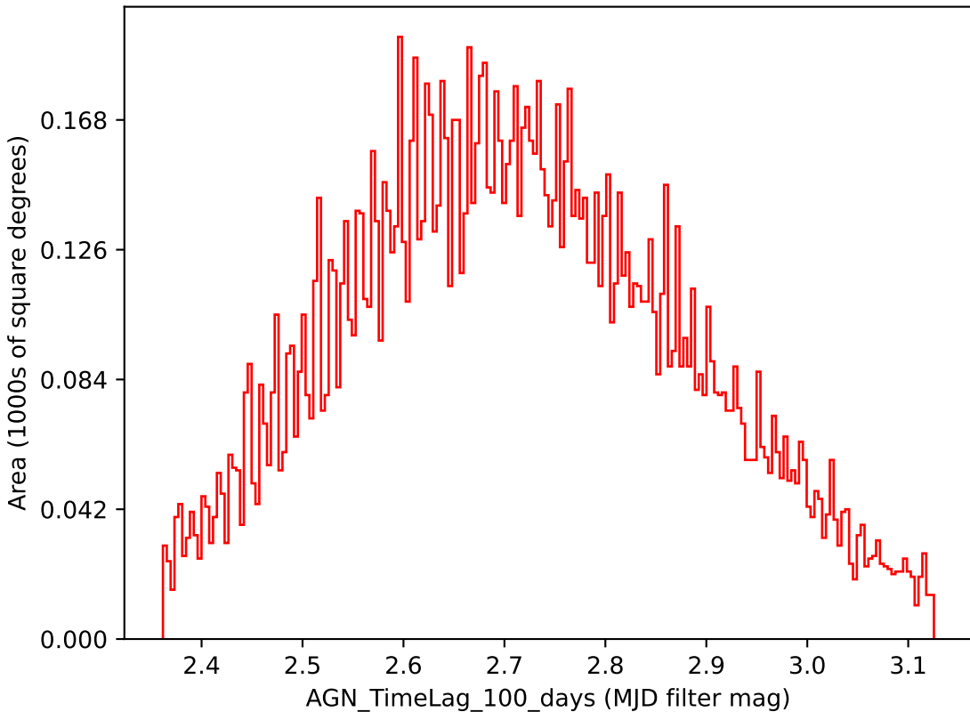
all_long_v3.4_10yrs i band: AGN_TimeLag_100_days
