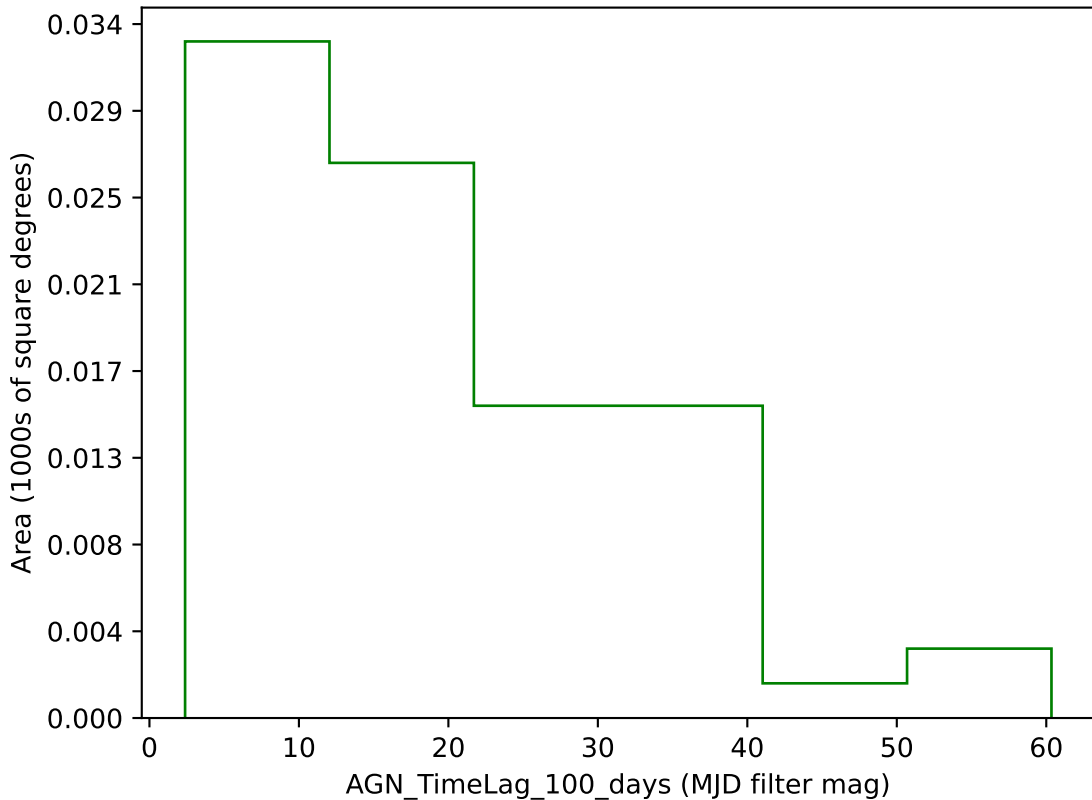
all_long_v3.4_10yrs g band: AGN_TimeLag_100_days
