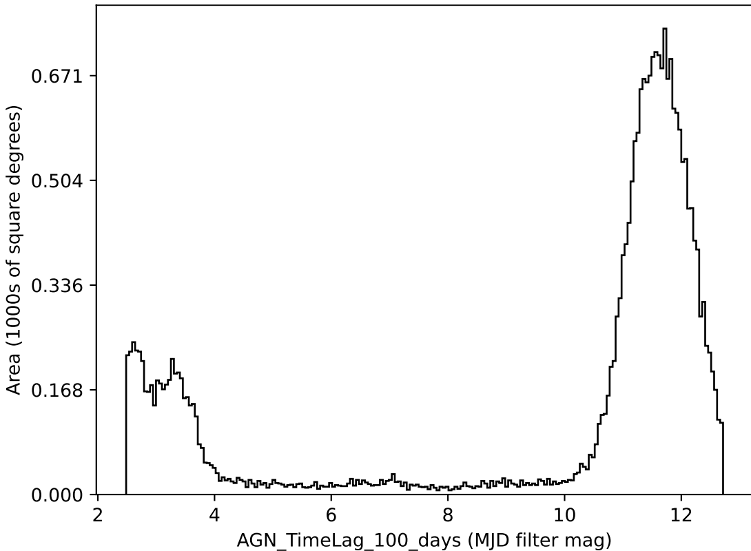
all_long_v3.4_10yrs all bands: AGN_TimeLag_100_days
