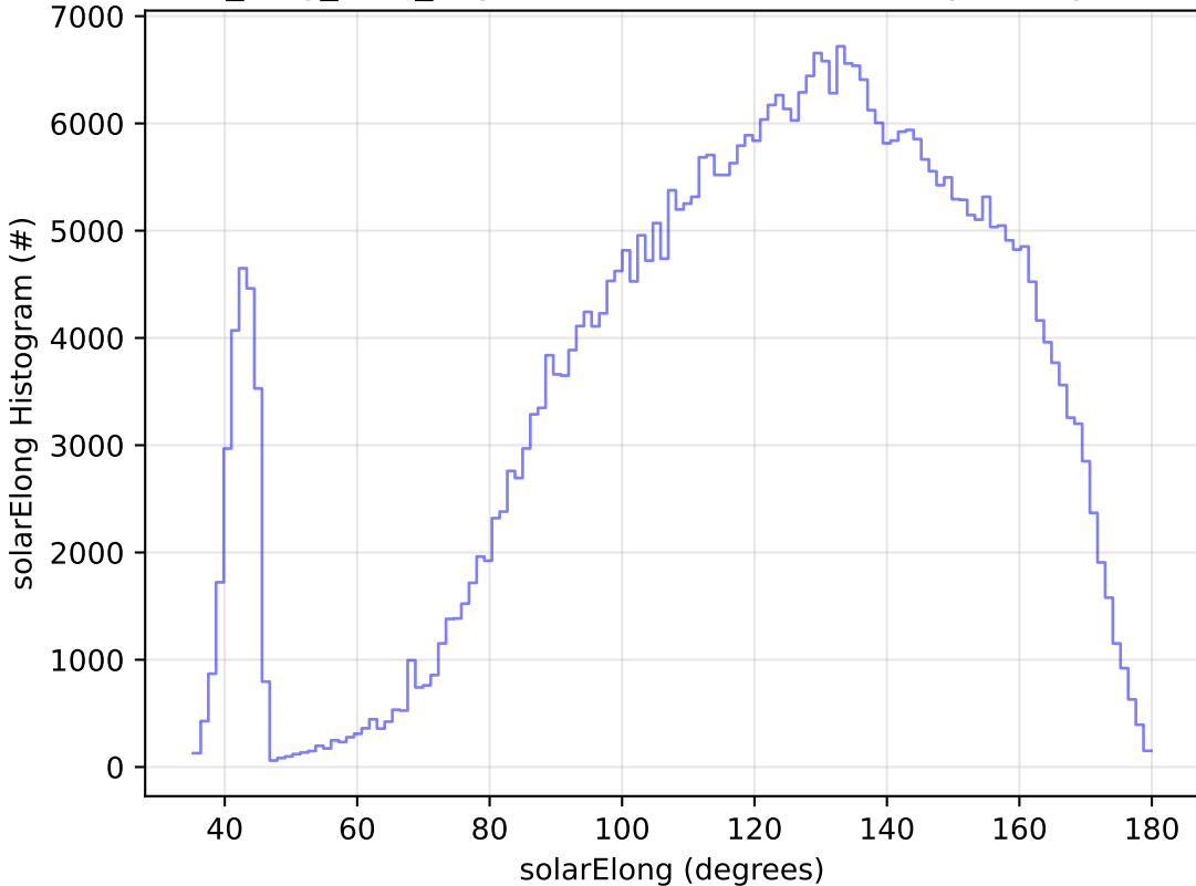
all_long_v3.4_10yrs WFD z band: solarElong Histogram
