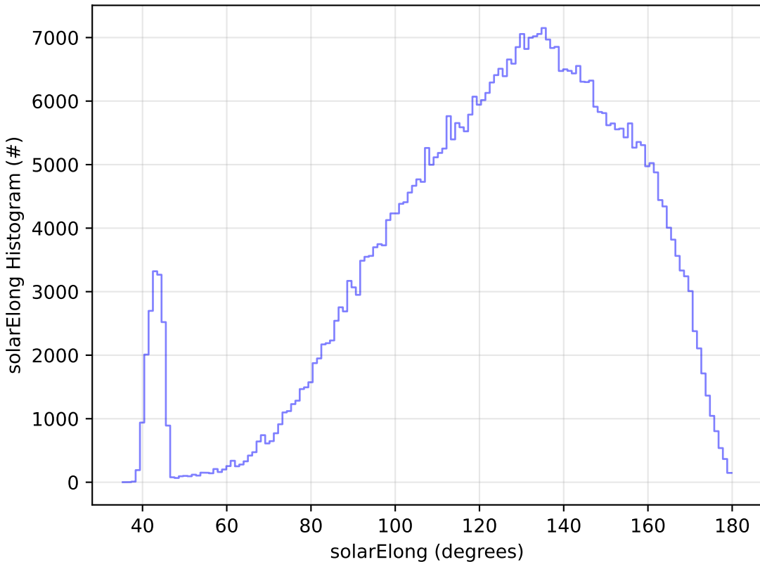
all_long_v3.4_10yrs WFD r band: solarElong Histogram
