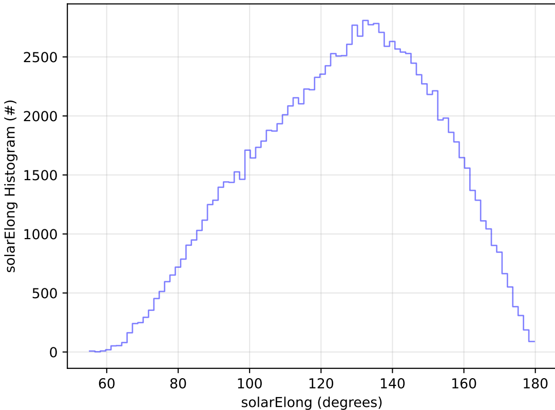
all_long_v3.4_10yrs All sky u band: solarElong Histogram
