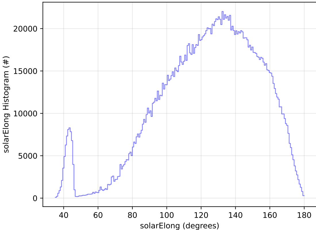
all_long_v3.4_10yrs All sky all bands: solarElong Histogram
