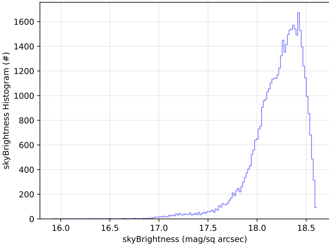
all_long_v3.4_10yrs Yr 1 y band: skyBrightness Histogram
