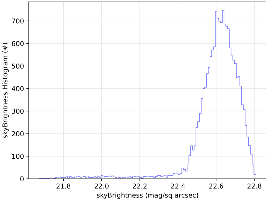
all_long_v3.4_10yrs Yr 1 u band: skyBrightness Histogram
