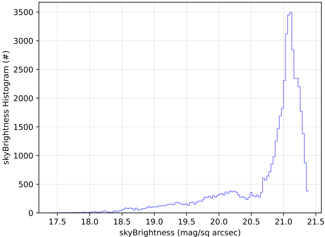
all_long_v3.4_10yrs Yr 1 r band: skyBrightness Histogram
