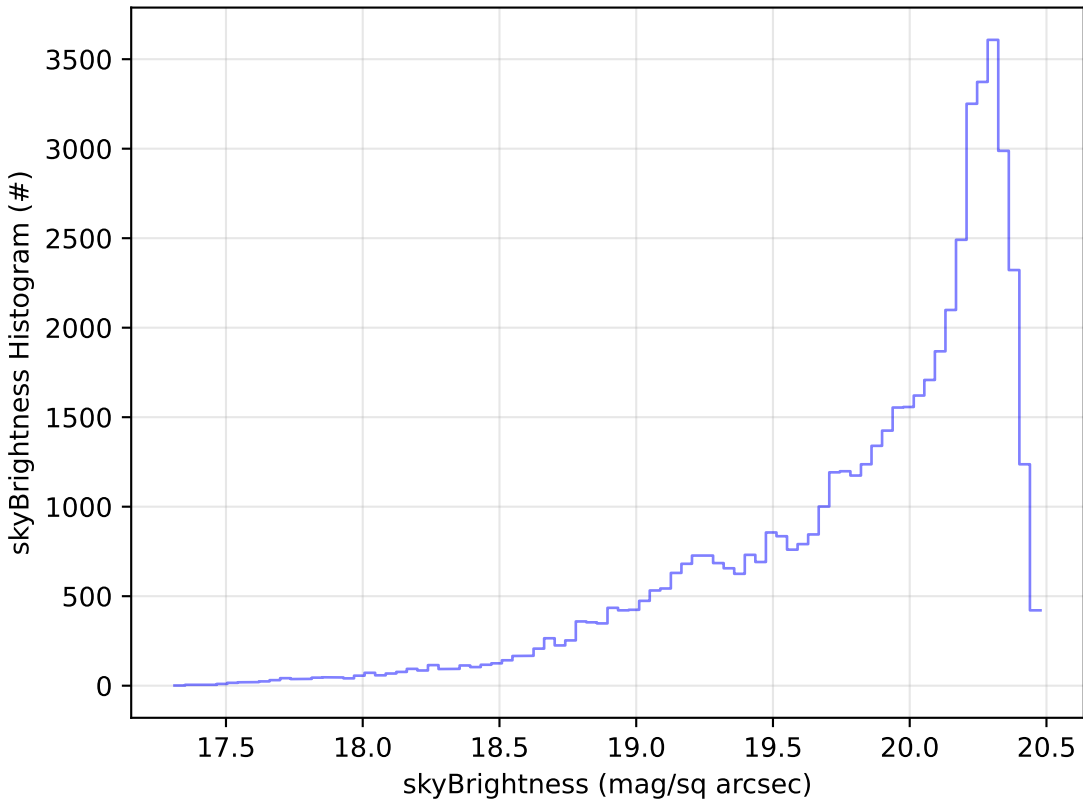
all_long_v3.4_10yrs Yr 1 i band: skyBrightness Histogram
