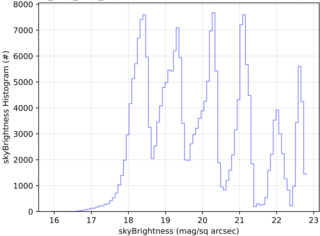
all_long_v3.4_10yrs Yr 1 all bands: skyBrightness Histogram
