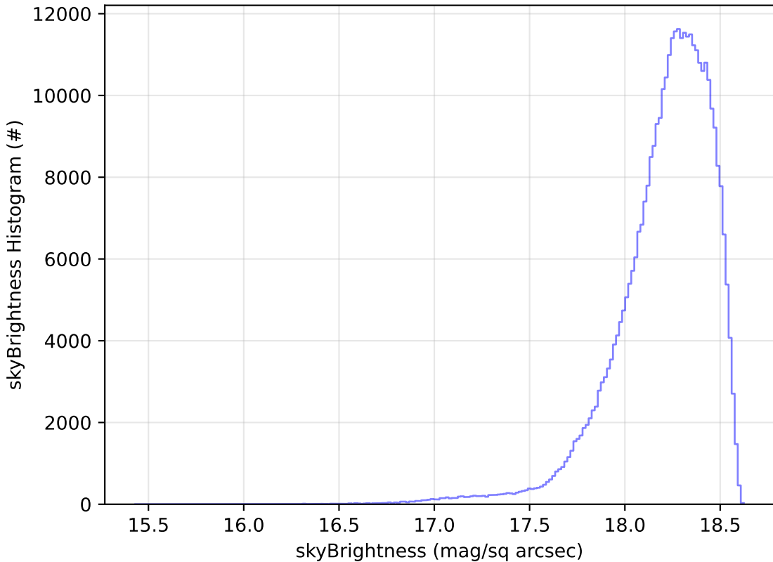
all_long_v3.4_10yrs WFD y band: skyBrightness Histogram
