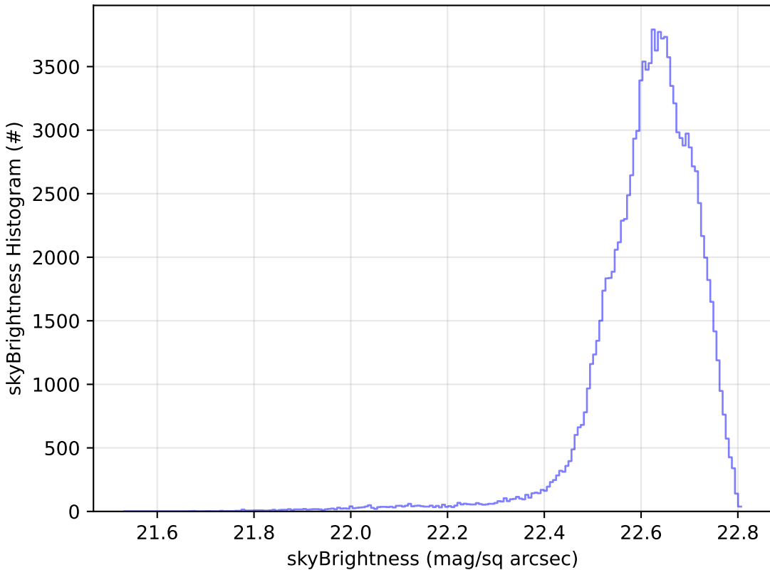
all_long_v3.4_10yrs WFD u band: skyBrightness Histogram
