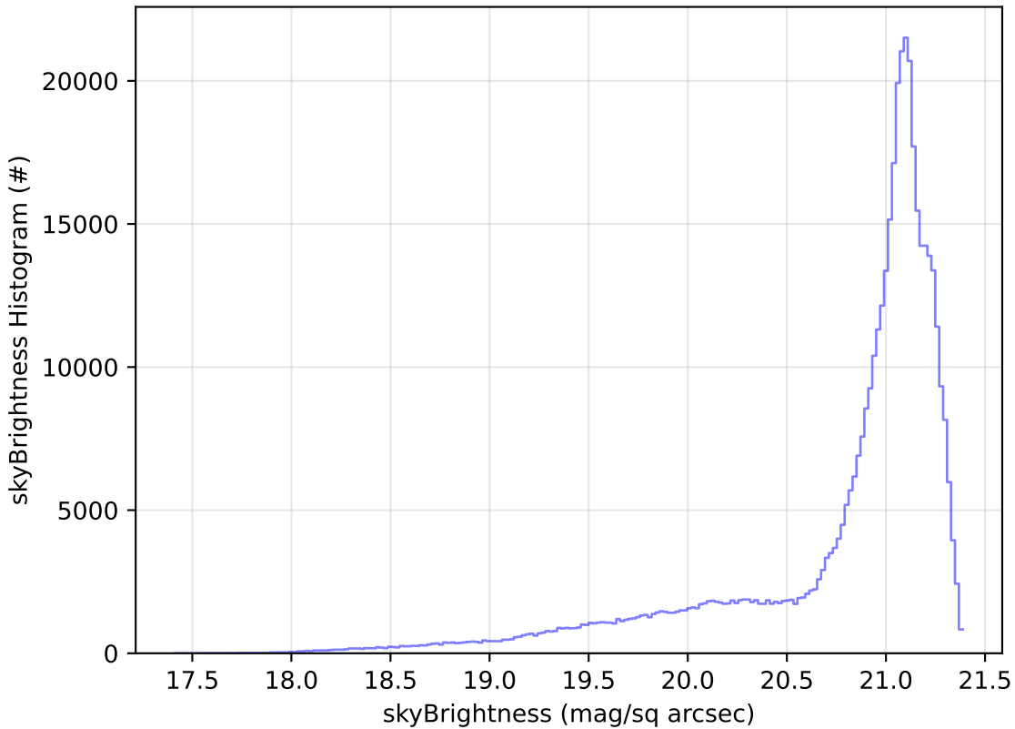
all_long_v3.4_10yrs WFD r band: skyBrightness Histogram
