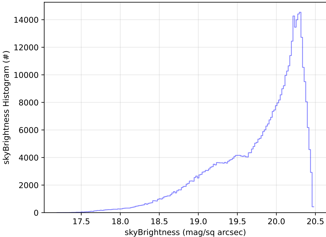
all_long_v3.4_10yrs WFD i band: skyBrightness Histogram
