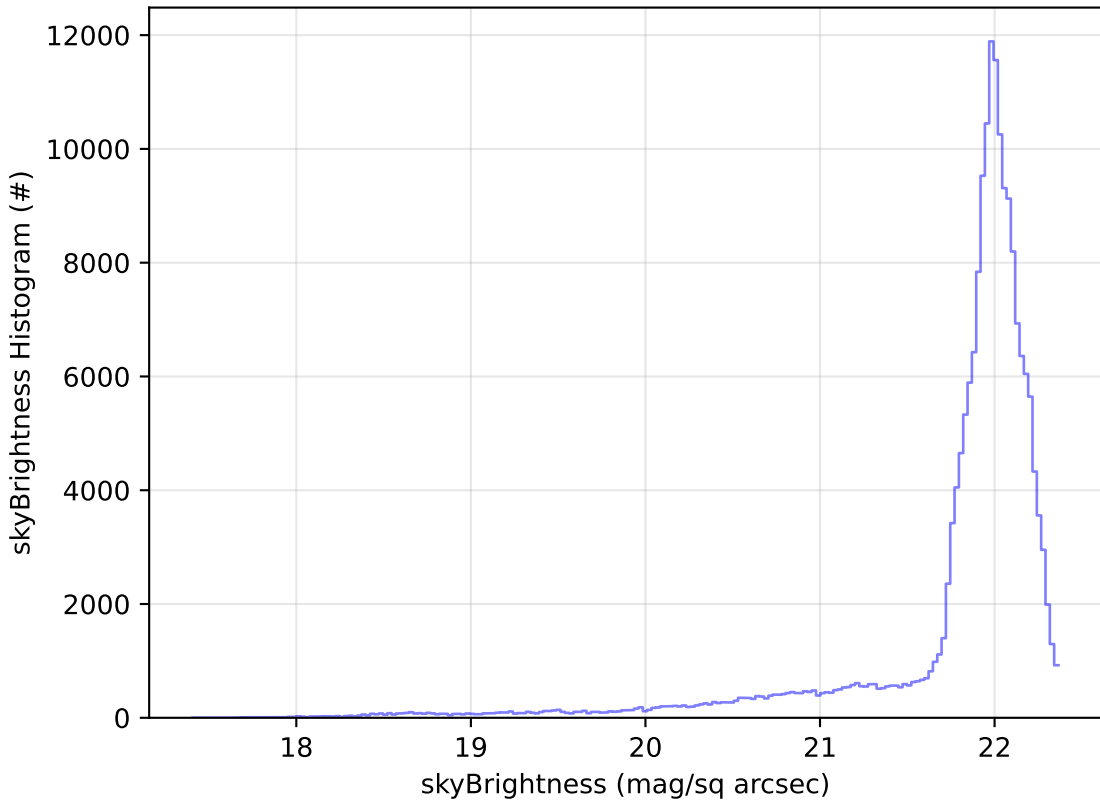
all_long_v3.4_10yrs WFD g band: skyBrightness Histogram
