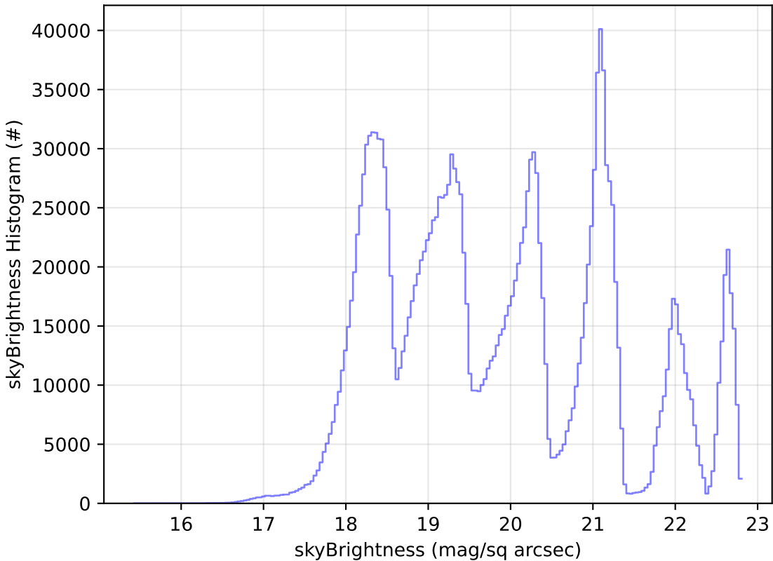
all_long_v3.4_10yrs WFD all bands: skyBrightness Histogram
