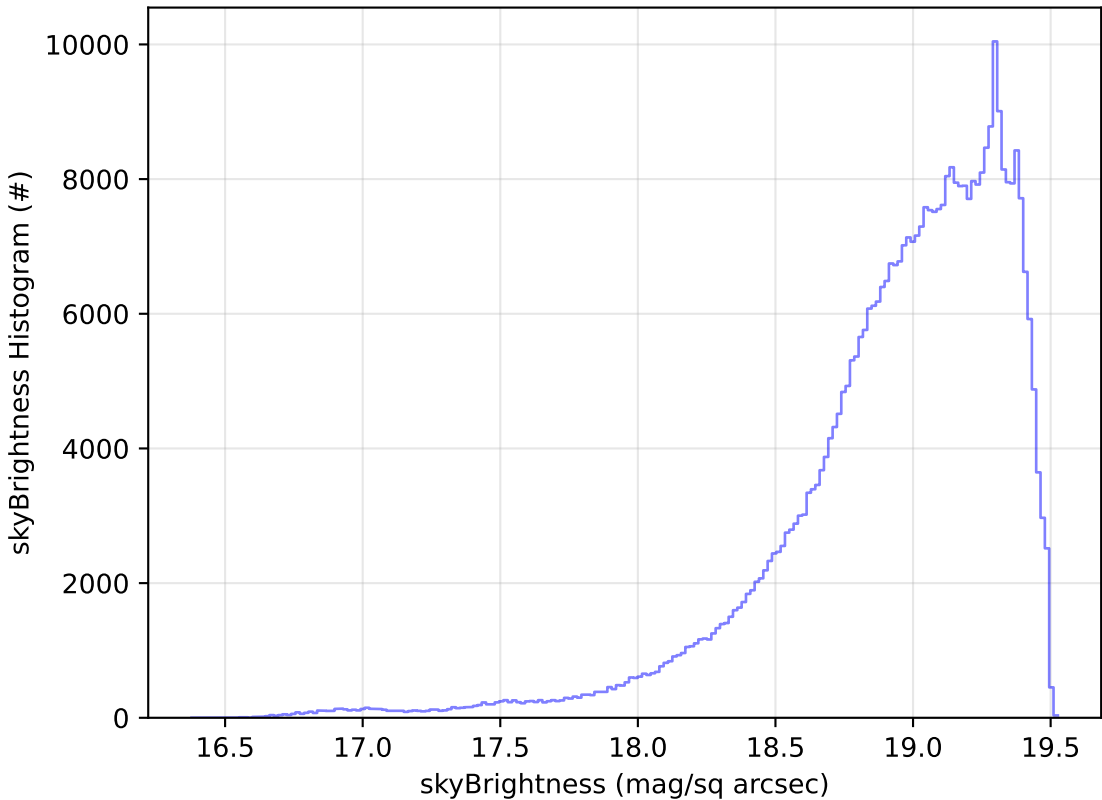
all_long_v3.4_10yrs All sky z band: skyBrightness Histogram
