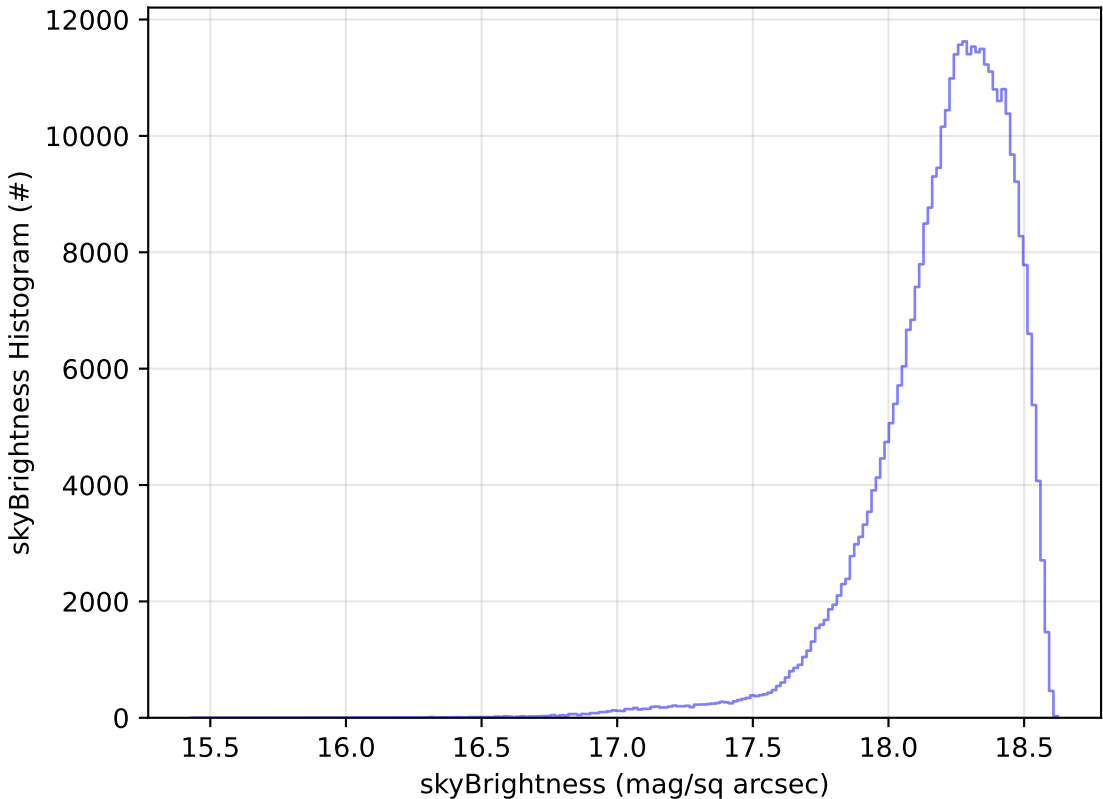
all_long_v3.4_10yrs All sky y band: skyBrightness Histogram
