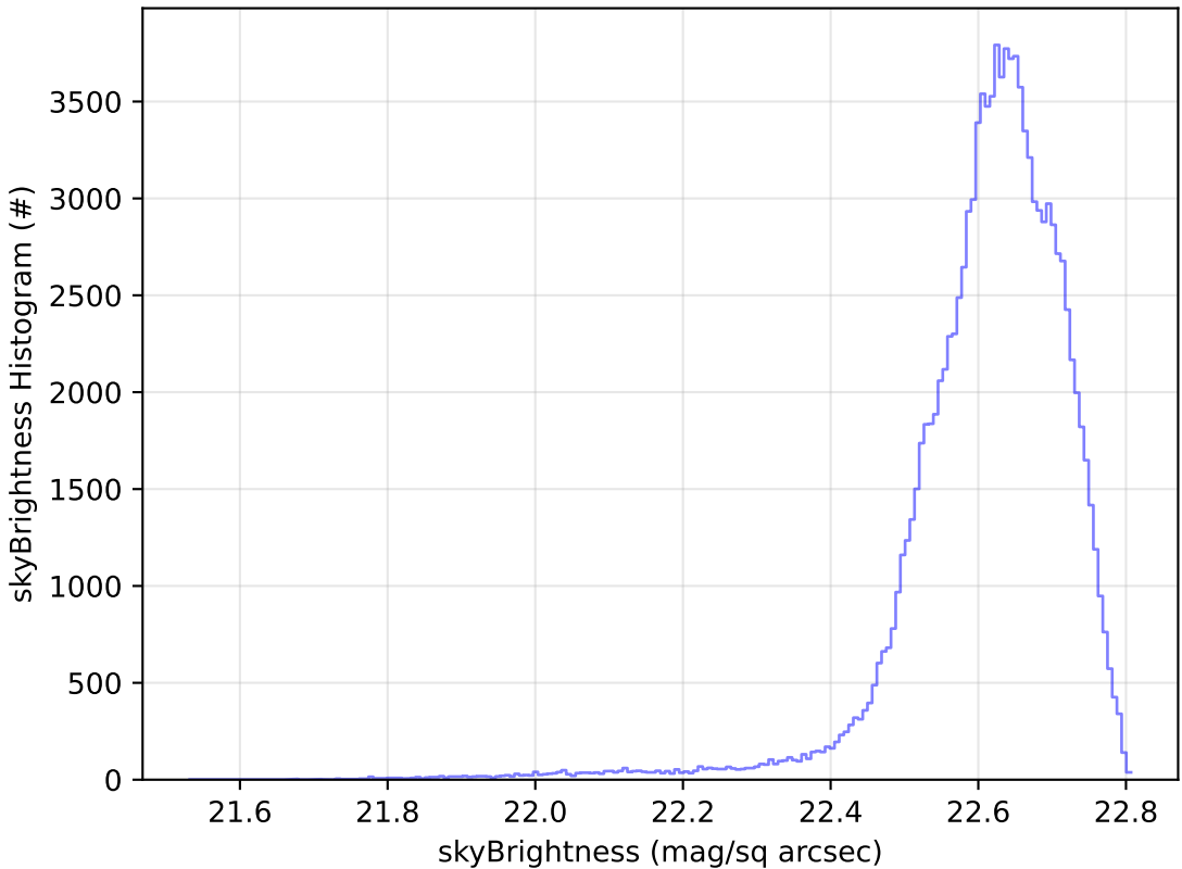
all_long_v3.4_10yrs All sky u band: skyBrightness Histogram
