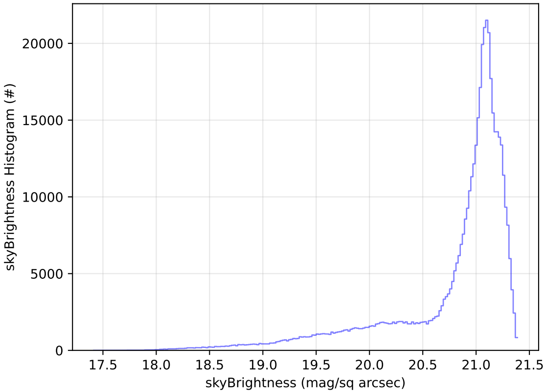
all_long_v3.4_10yrs All sky r band: skyBrightness Histogram
