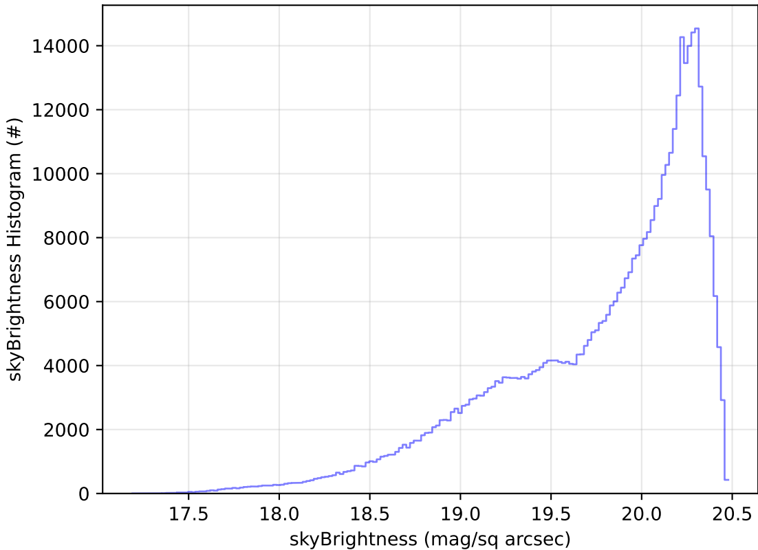
all_long_v3.4_10yrs All sky i band: skyBrightness Histogram
