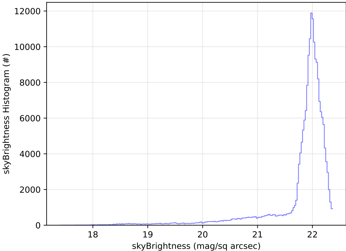
all_long_v3.4_10yrs All sky g band: skyBrightness Histogram
