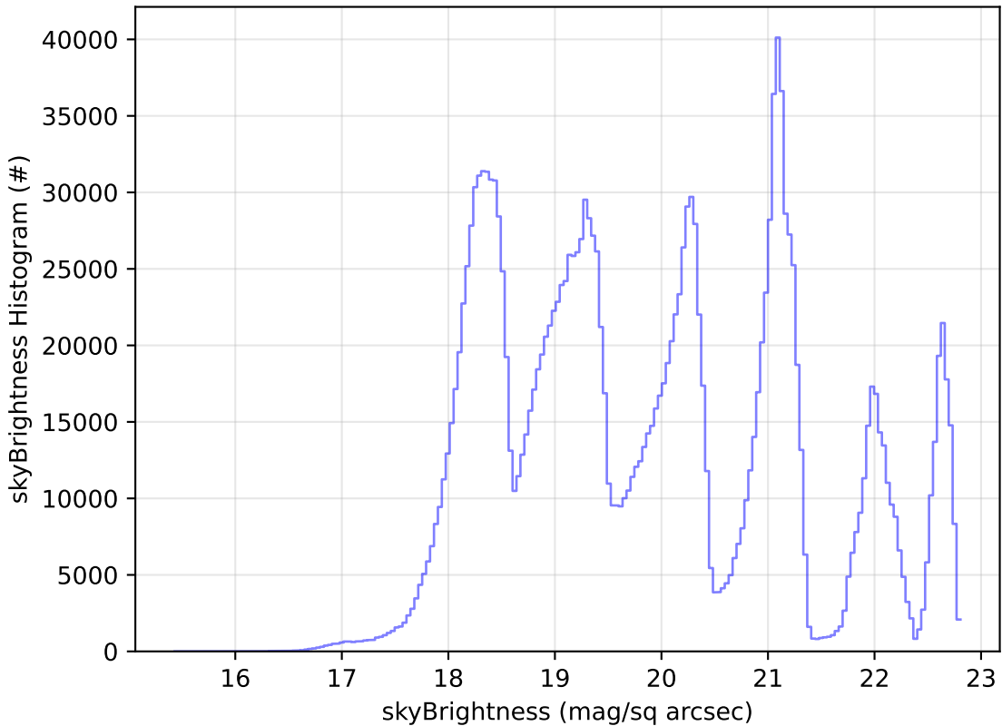
all_long_v3.4_10yrs All sky all bands: skyBrightness Histogram
