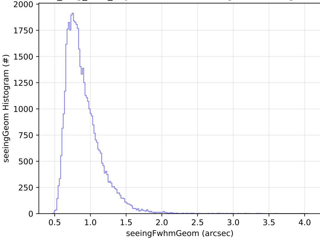
all_long_v3.4_10yrs Yr 1 z band: seeingGeom Histogram
