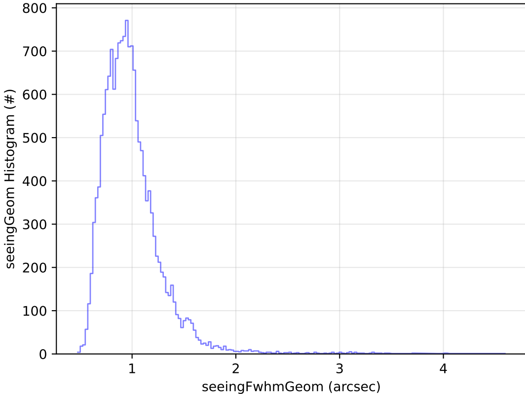
all_long_v3.4_10yrs Yr 1 u band: seeingGeom Histogram
