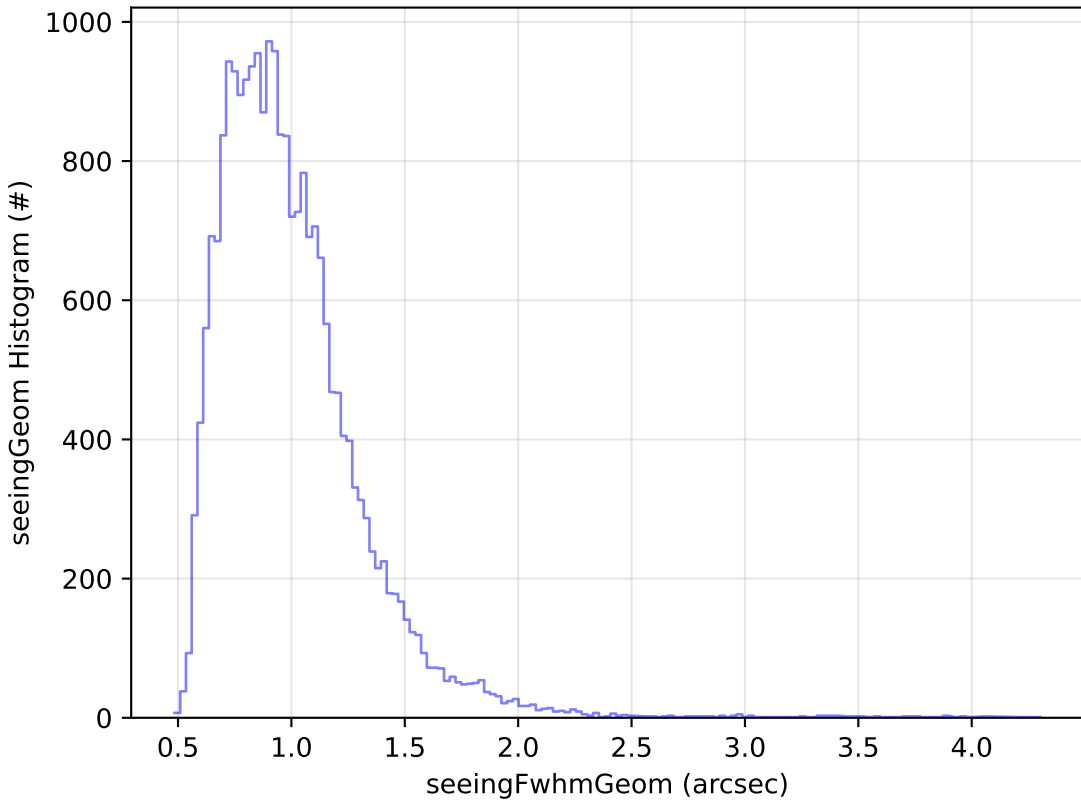
all_long_v3.4_10yrs Yr 1 g band: seeingGeom Histogram
