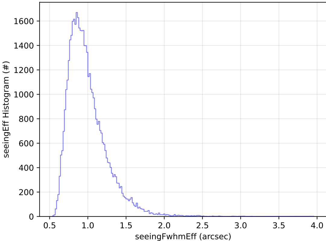
all_long_v3.4_10yrs Yr 1 y band: seeingEff Histogram
