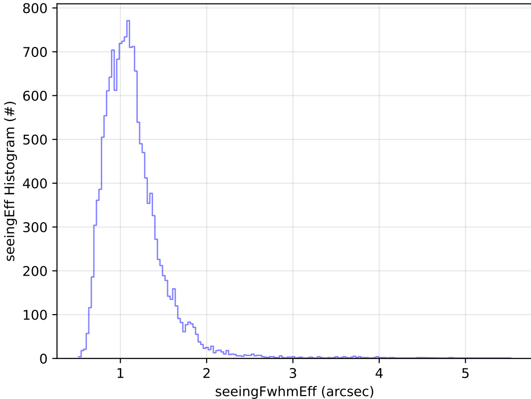
all_long_v3.4_10yrs Yr 1 u band: seeingEff Histogram
