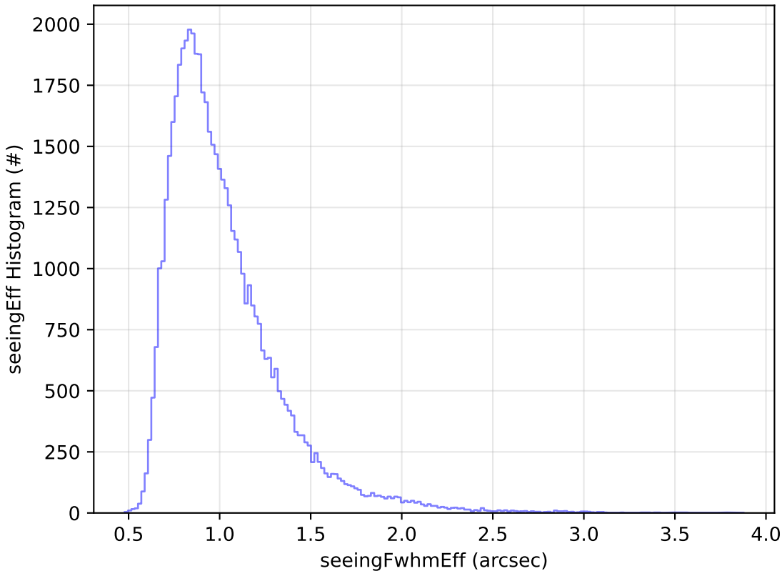
all_long_v3.4_10yrs Yr 1 i band: seeingEff Histogram
