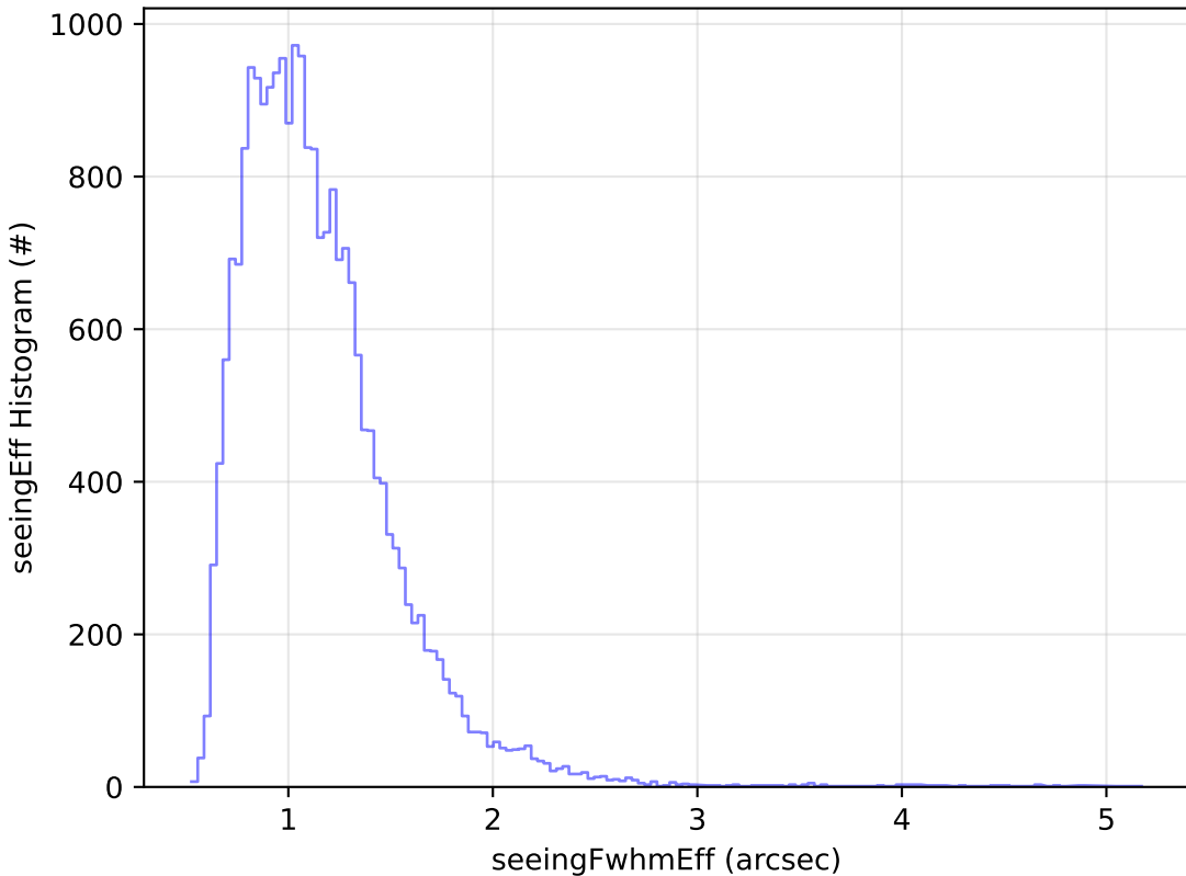
all_long_v3.4_10yrs Yr 1 g band: seeingEff Histogram
