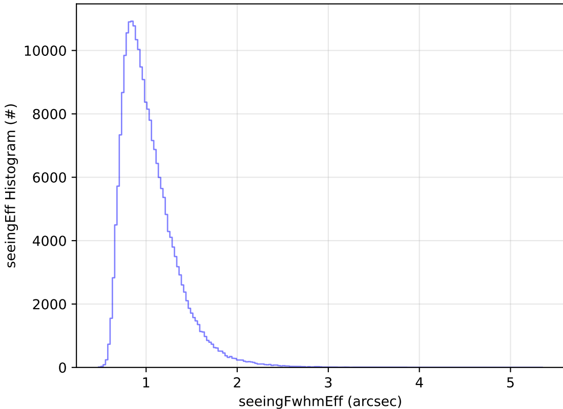
all_long_v3.4_10yrs Yr 1 all bands: seeingEff Histogram
