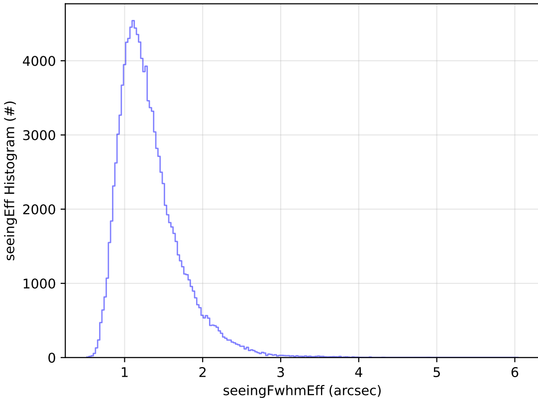
all_long_v3.4_10yrs WFD u band: seeingEff Histogram
