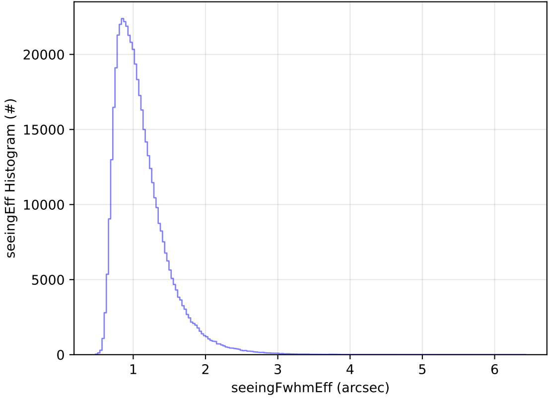
all_long_v3.4_10yrs WFD i band: seeingEff Histogram
