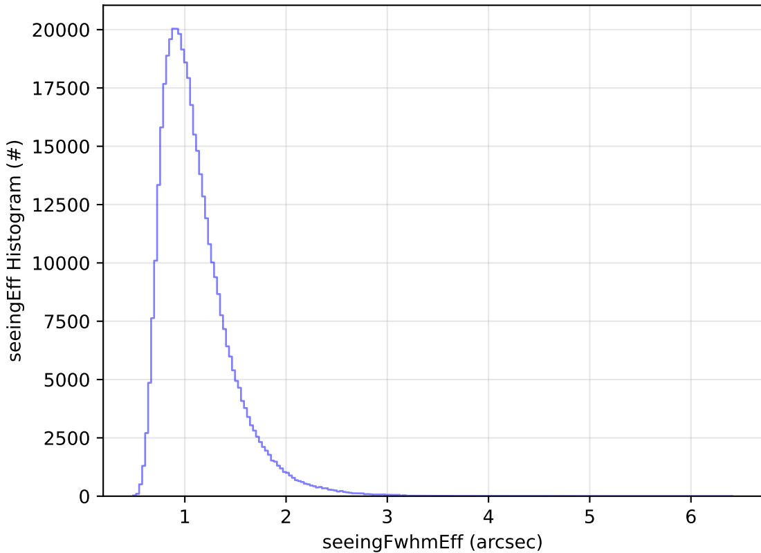
all_long_v3.4_10yrs All sky z band: seeingEff Histogram
