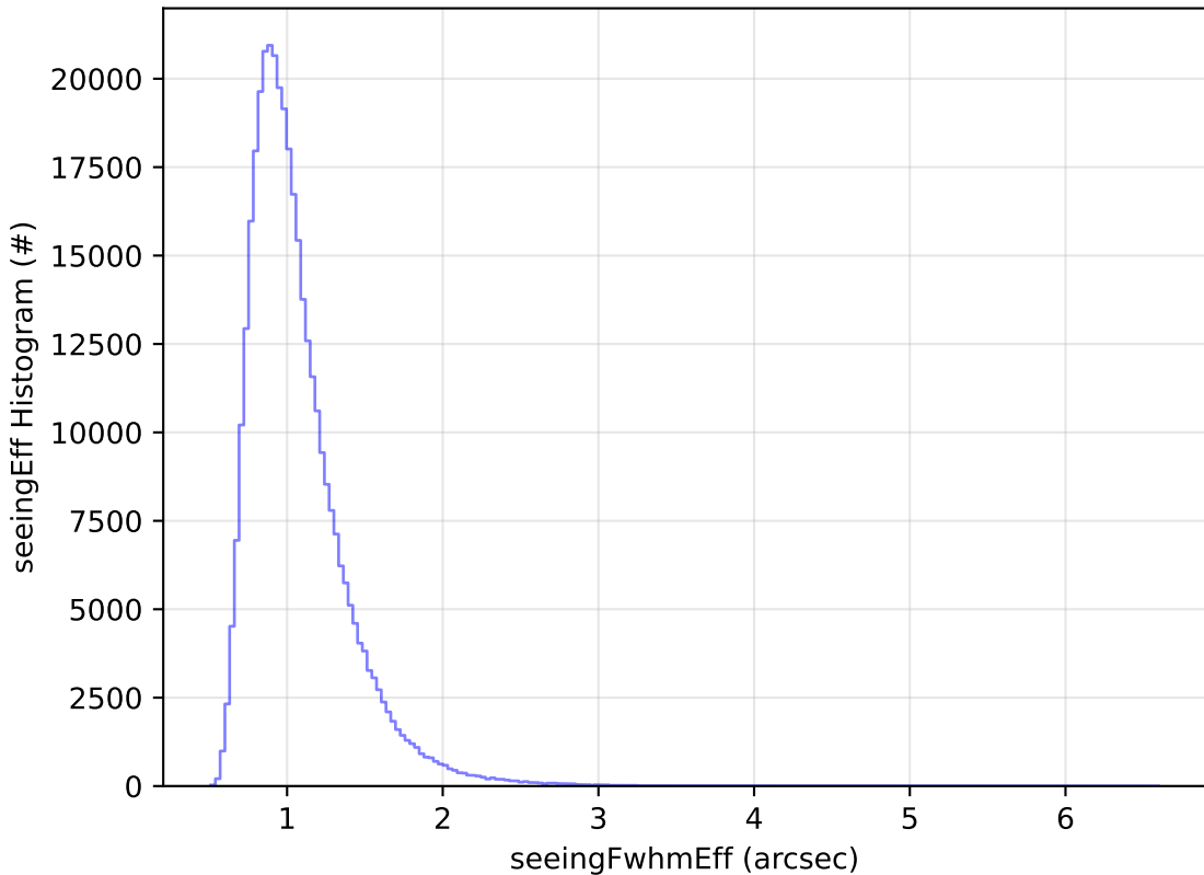
all_long_v3.4_10yrs All sky y band: seeingEff Histogram
