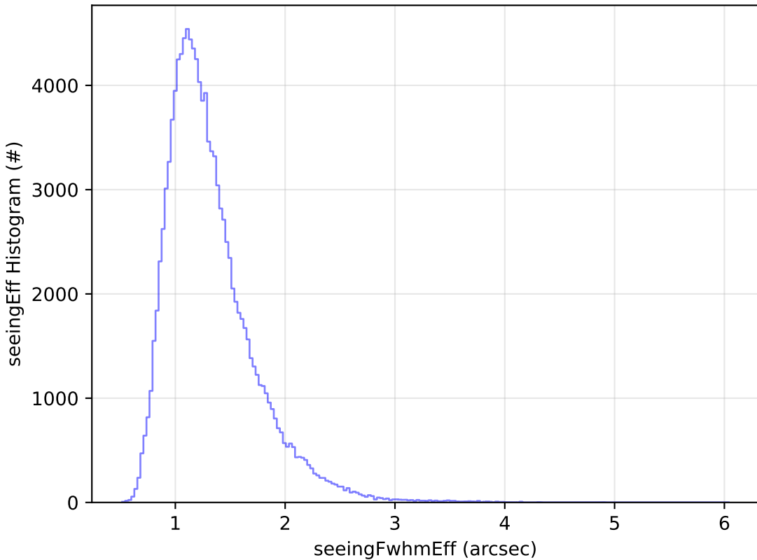
all_long_v3.4_10yrs All sky u band: seeingEff Histogram
